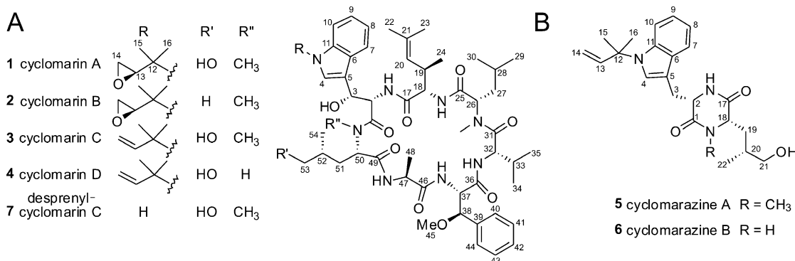
Figure 1. Structures of cyclomarins ( 1–4, 7 ) and cyclomarazine ( 5 and 6 ) cyclic peptides from Salinispora arenicola CNS-205 and Streptomyces sp. CNB-982.
